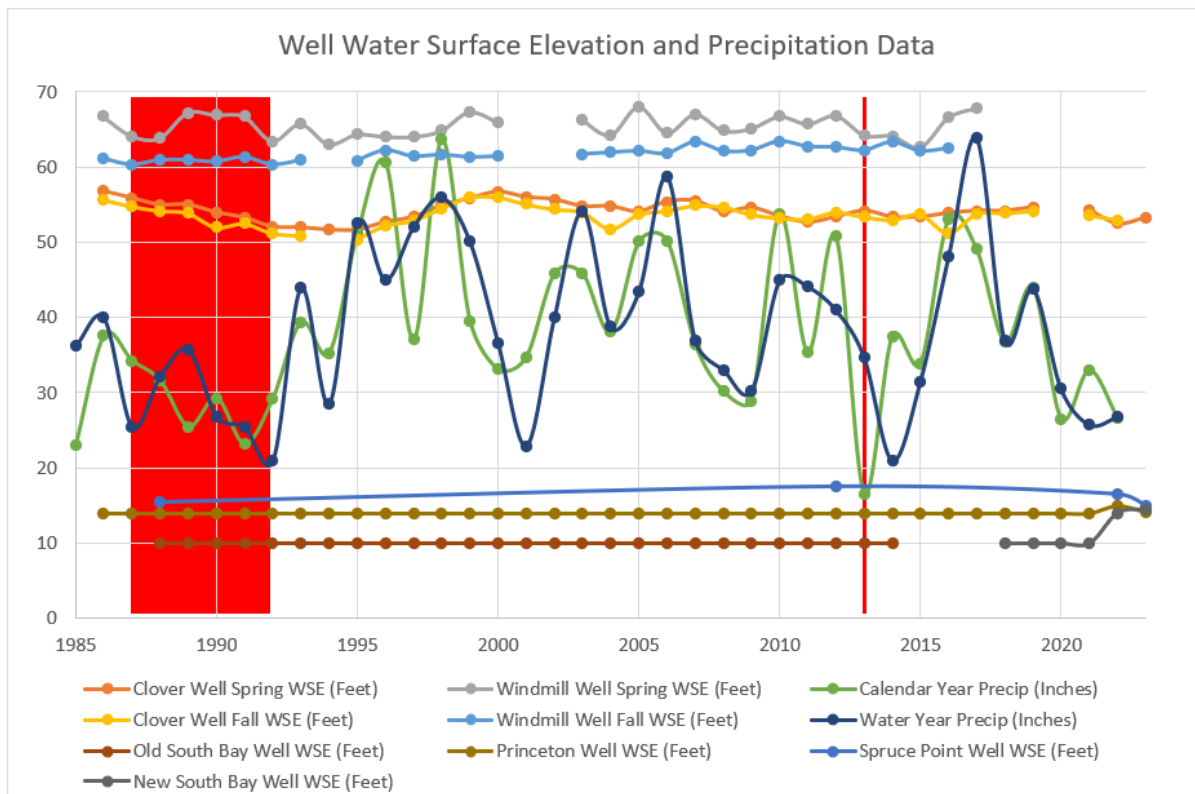
Figure 1: Water surface elevation and precipitation data for the Eureka Plain Basin between 1985 and 2023
